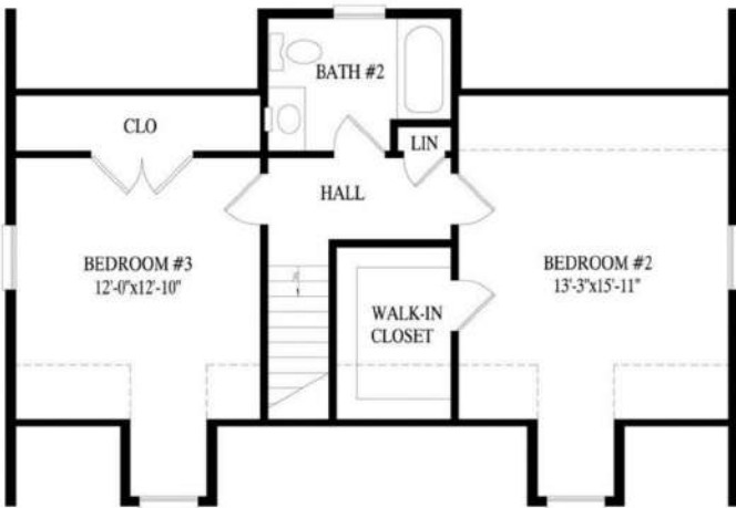
Proposed 2nd Floor - 674 sq. ft.
